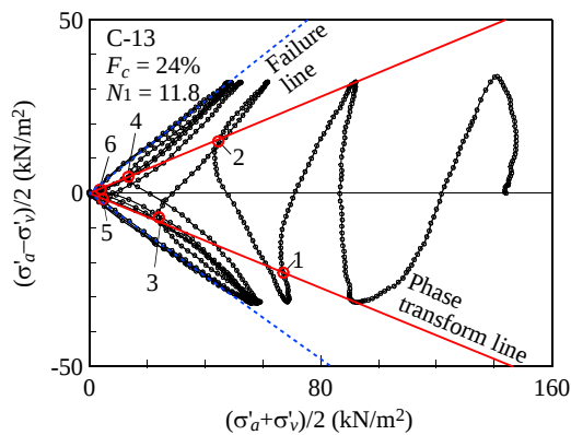
(a) Effective stress path
