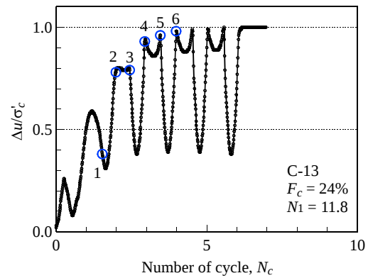
(b) Excess porewater pressure vs. number of cycles
