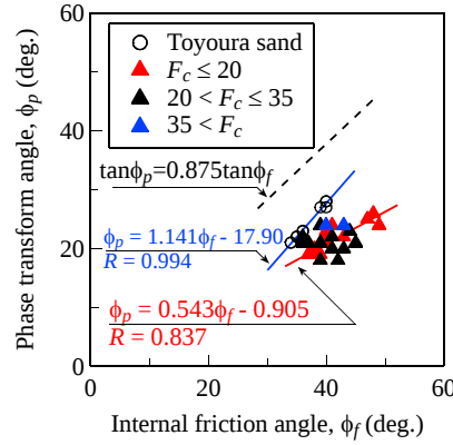
Fig. 6. Internal friction angle vs. phase transform angle
